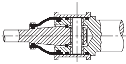
CROSS SECTION DRAWING OF MULTIPLE PIN & BUSH UNIVERSAL JOINT
