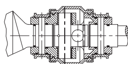
CROSS SECTIONAL DRAWING OF CARDON JOINT
