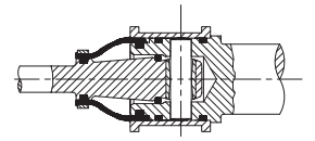
CROSS SECTION DRAWING OF PIN & BUSH UNIVERSAL JOINT
