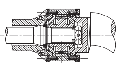
CROSS SECTIONAL DRAWING OF GEAR JOINT
